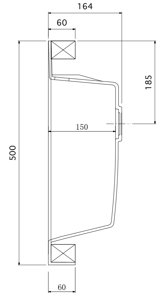
Sec A - A
